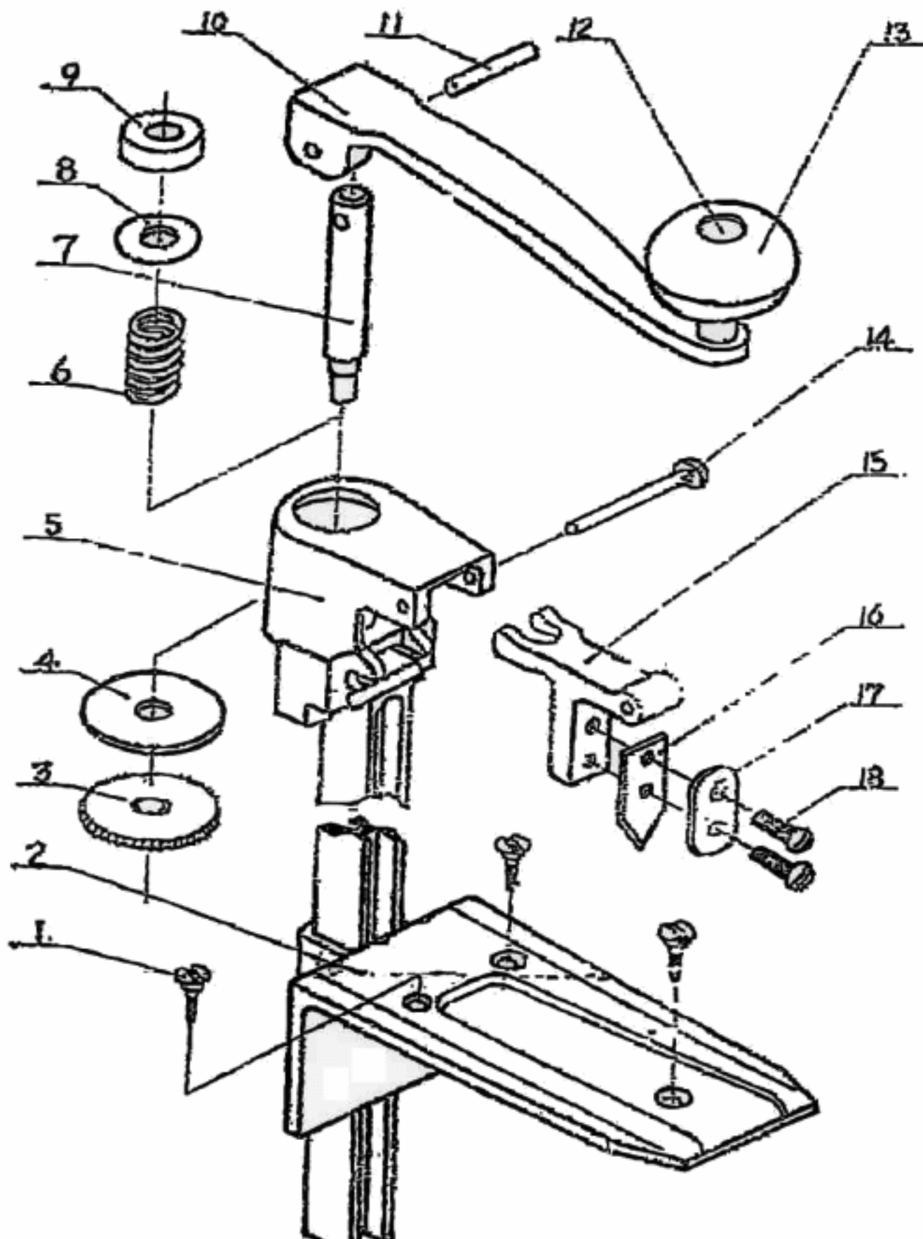
1. Screw 2. Base 3. Gear 4. Gear spacer 5. Body 6. Spring 7. Arbor 8. Spring Washer 9. Bushing 10. Handle 11. Handle Pin 12. Knob rivet 13. Knob 14. Knife Holder Pin 15. Knife Holder 16. Knife 17. Knife spacer 18. Screw
